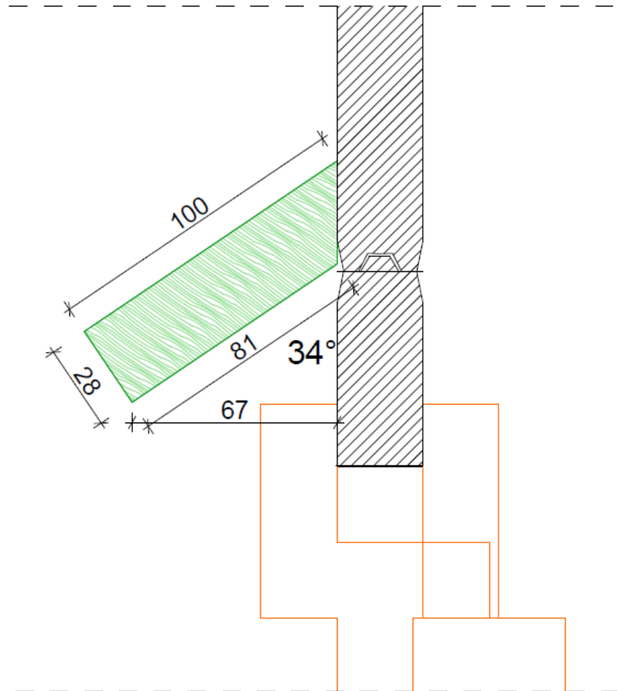
Drip cap over window/door
