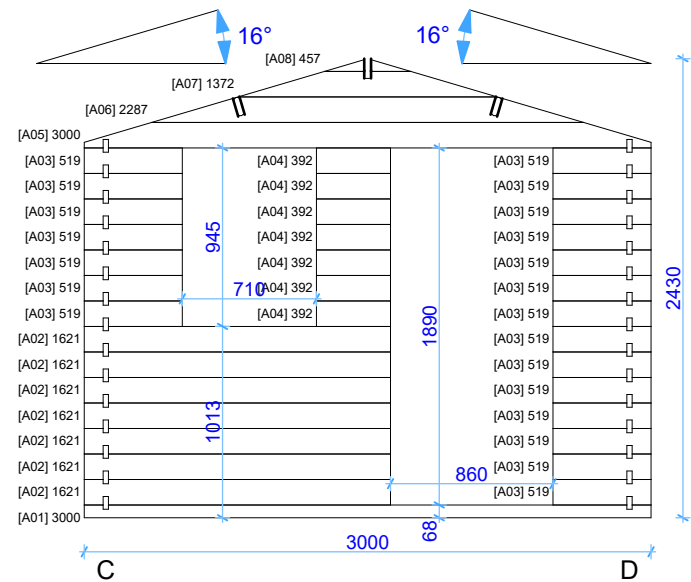
Wall A 1:40
