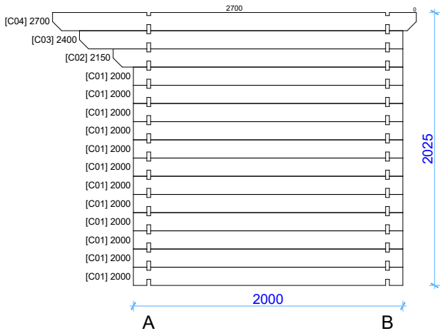
Wall C 1:40
