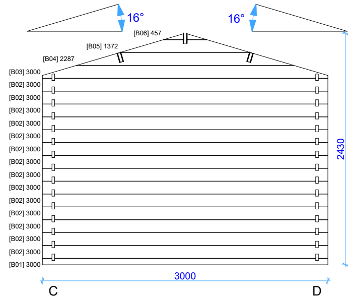
Wall B 1:40
