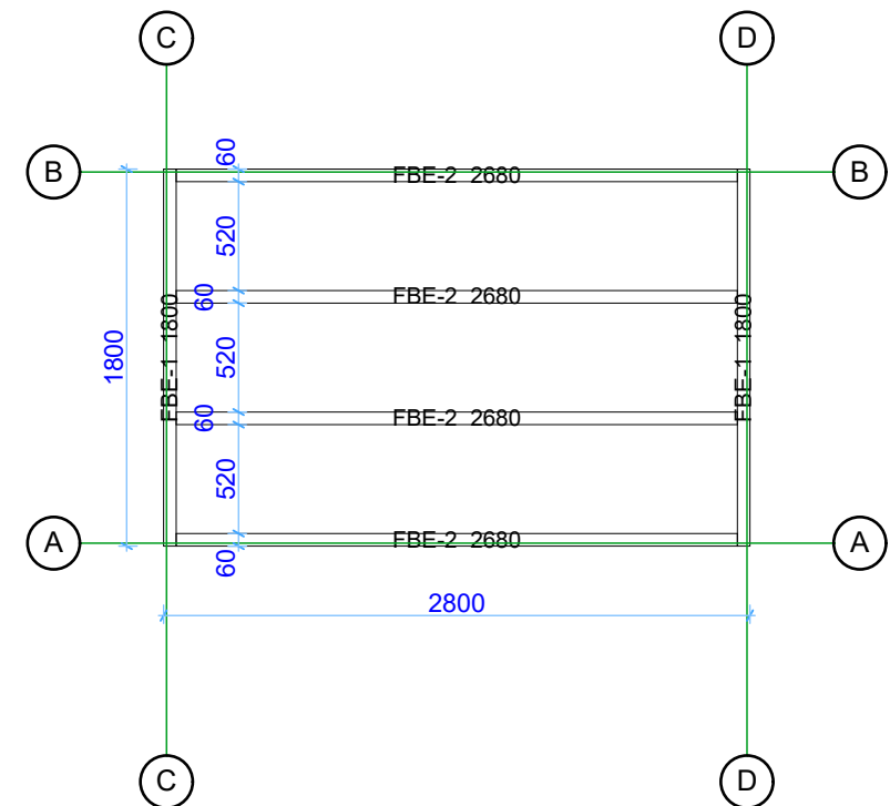
Floor bearers
