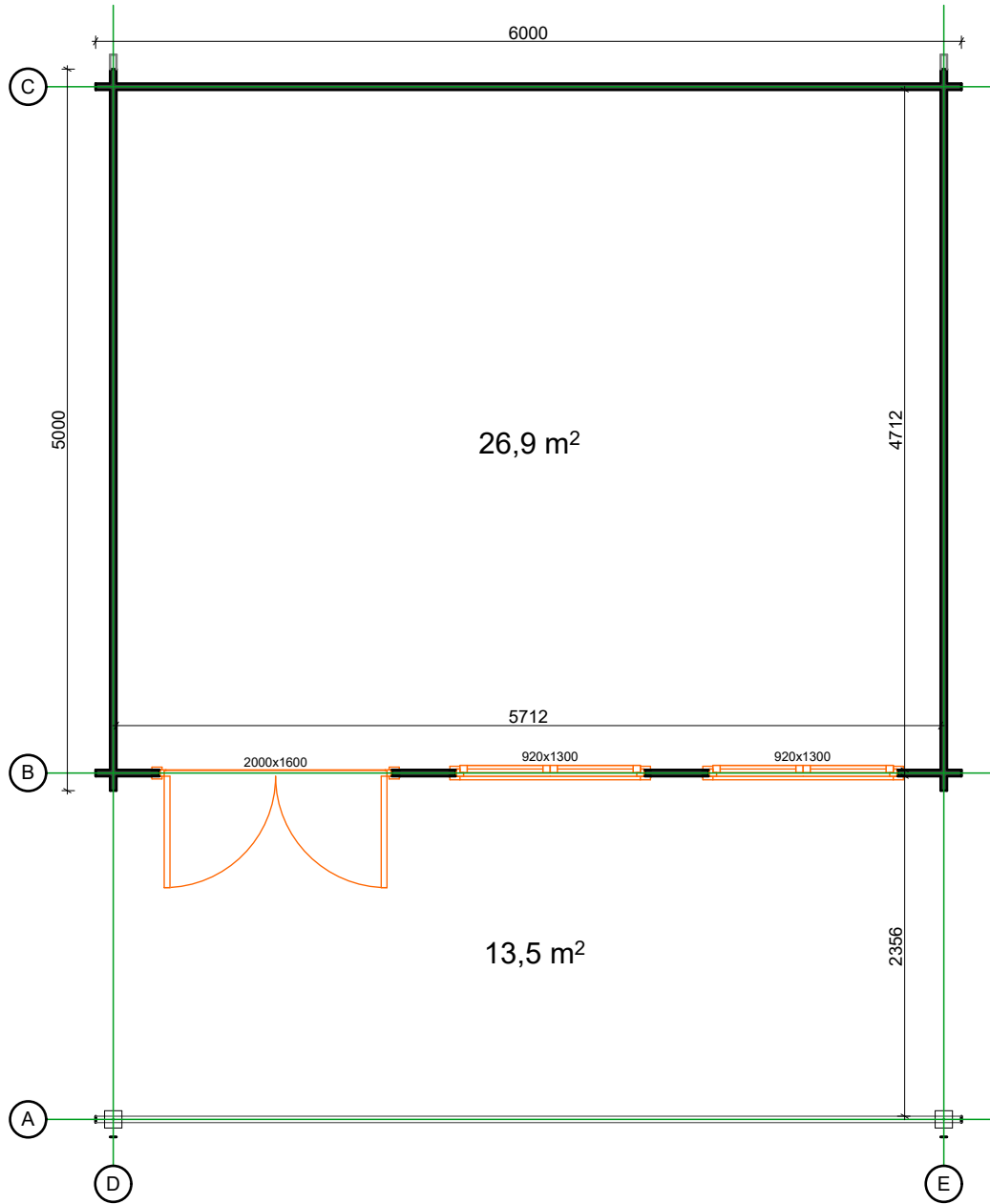
Floor plan 1:50
