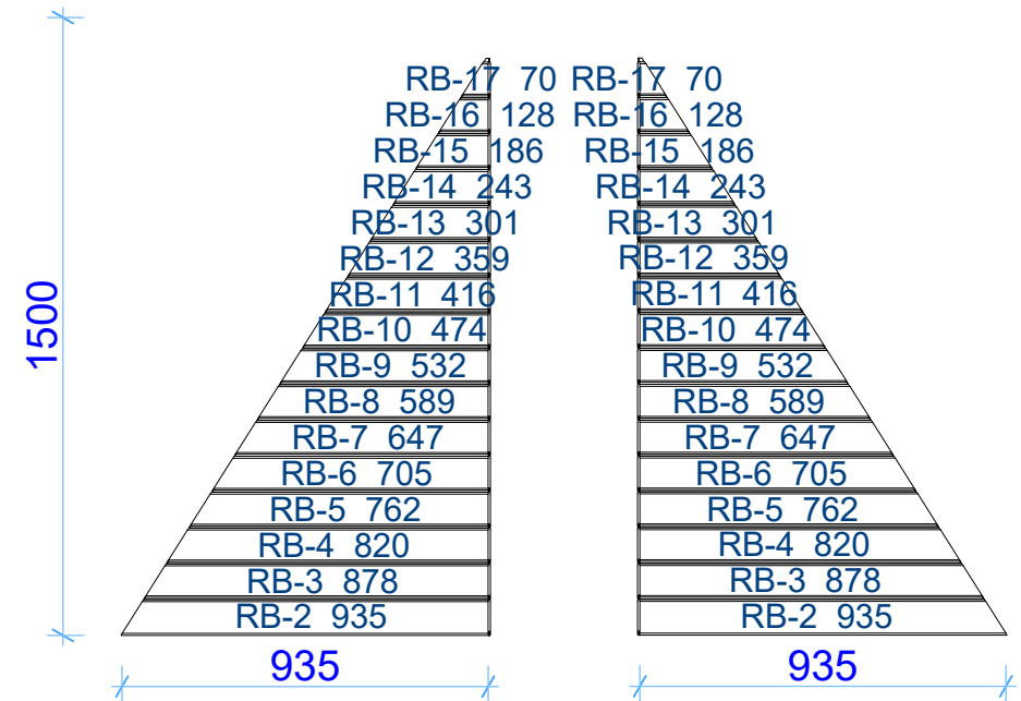
Roof boards
