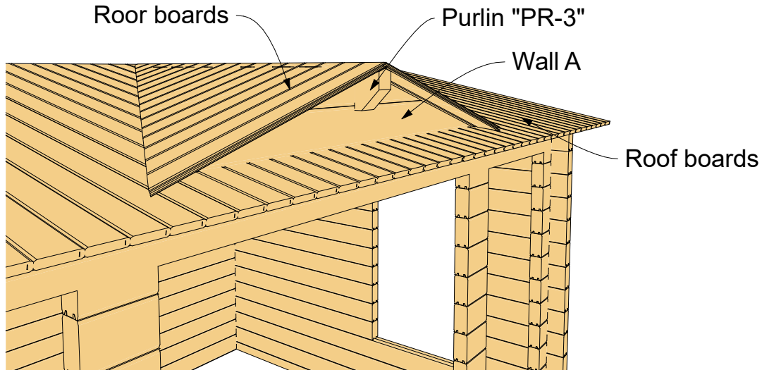
Roof boards
