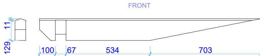
Purlin "PR-3"
