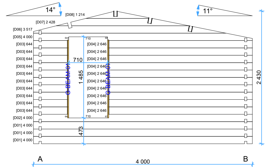
Wall D
