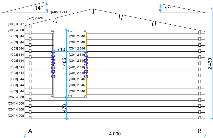
Wall C
