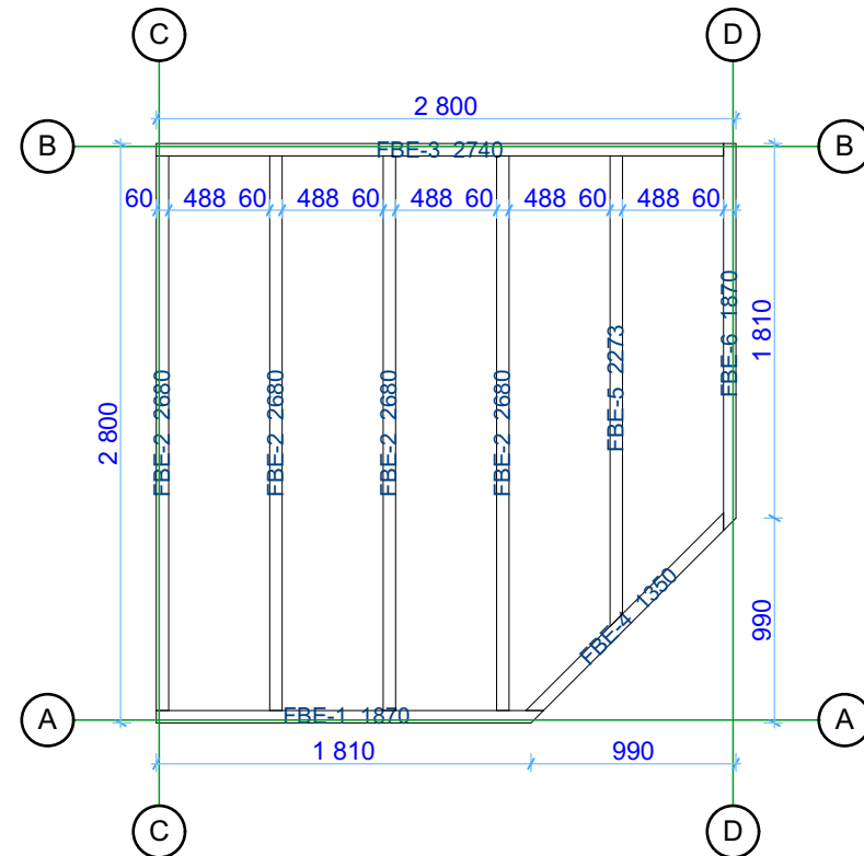
Floor bearers
