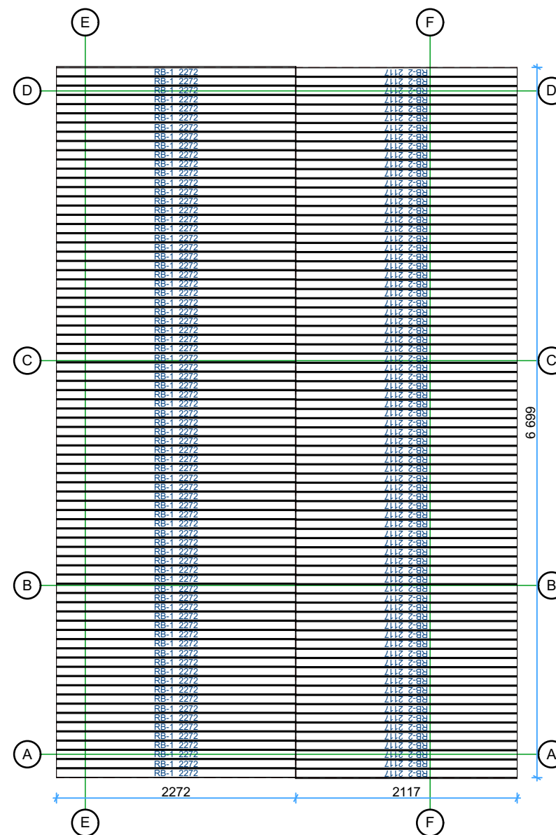
Roof boards
