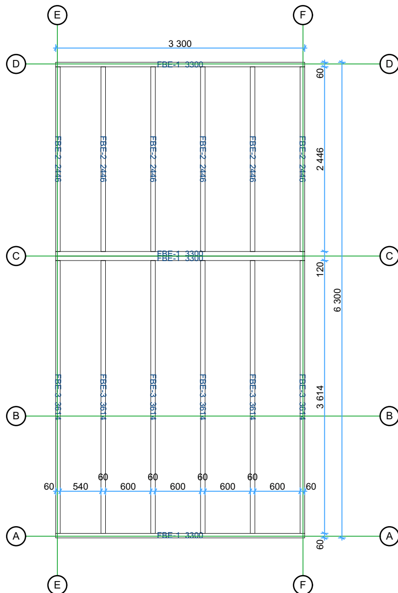
Floor bearer
