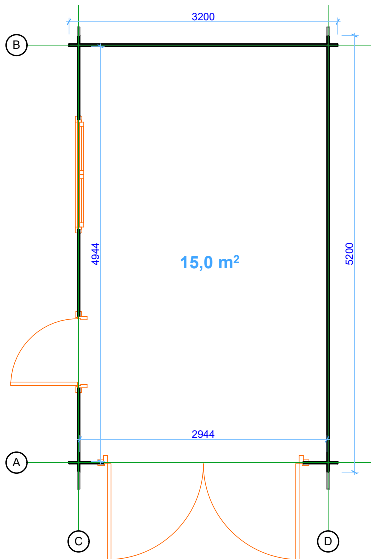
Floor plan
