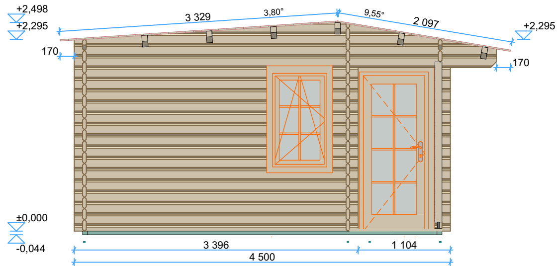
Left Elevation
