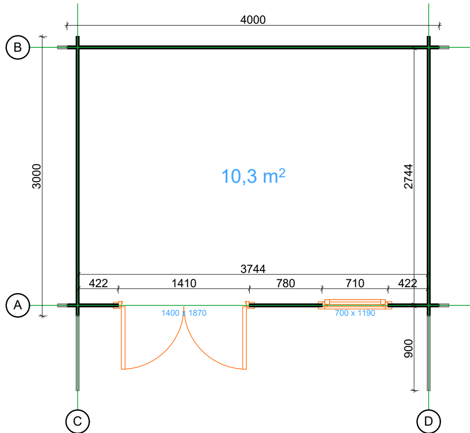
Floor plan 1:40
