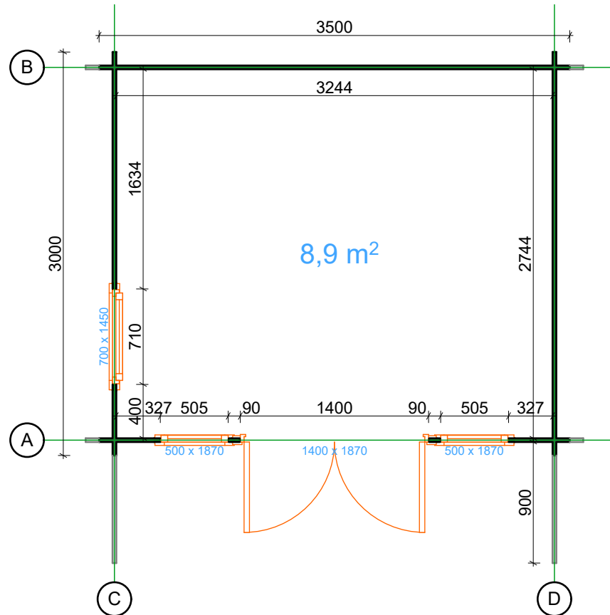
Floor plan 1:40
