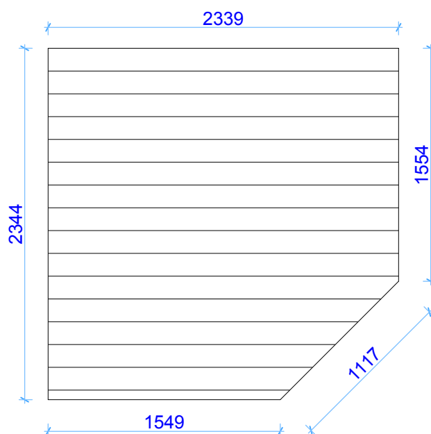
Floor boards
