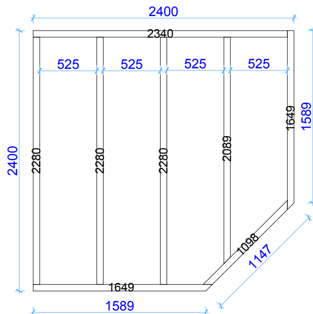
Floor bearers
