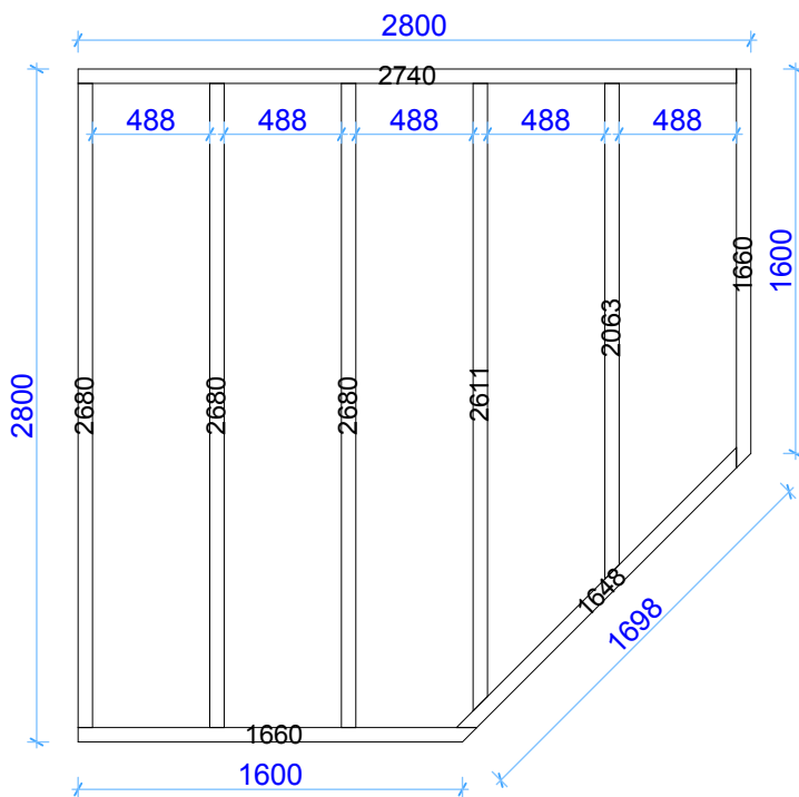
Floor bearers
