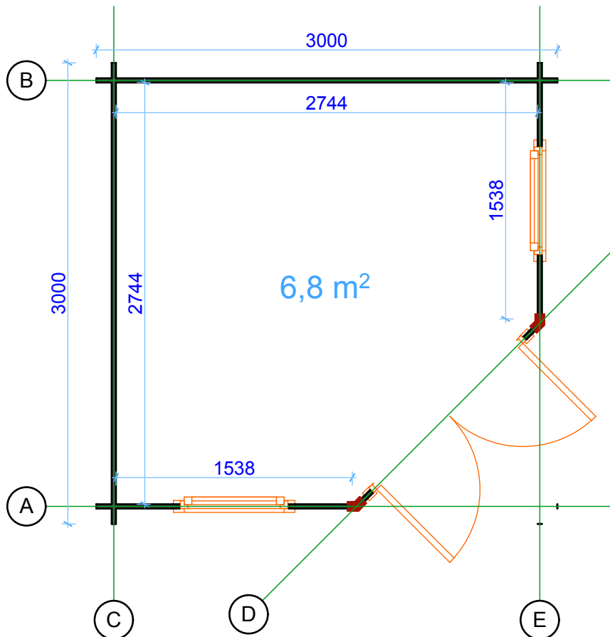
Floor plan
