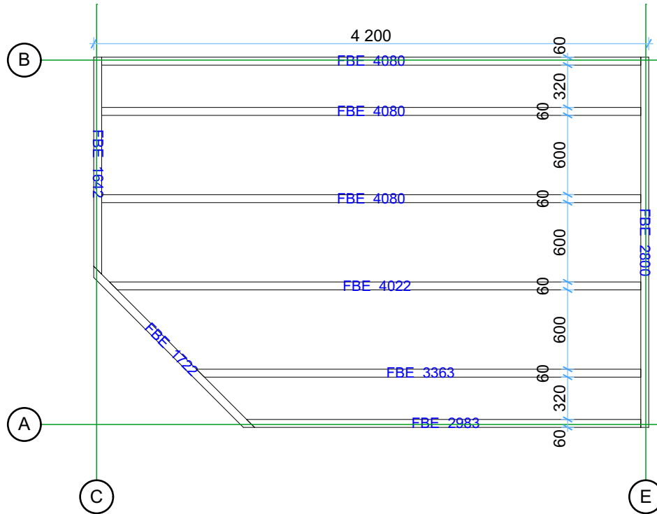
Floor bearers
